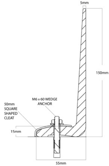
150mm FlexiBaffle Dimensions.
