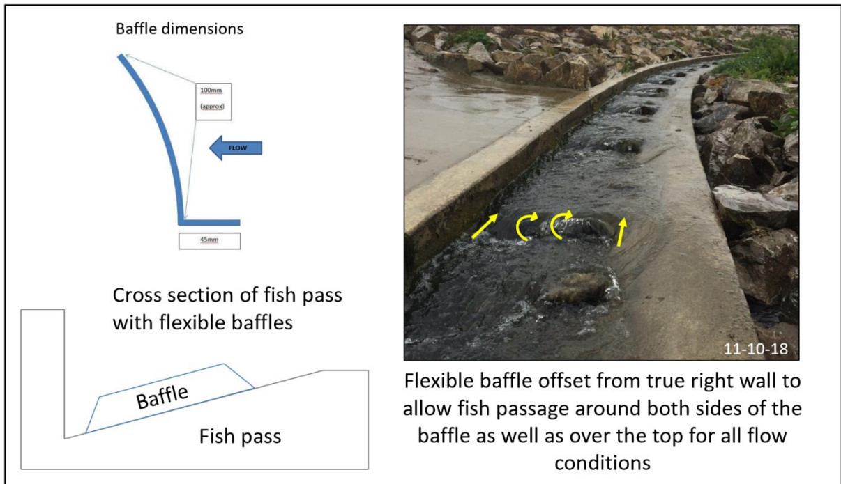
Figure 3. Flexible baffle dimensions and positions within the fish pass
