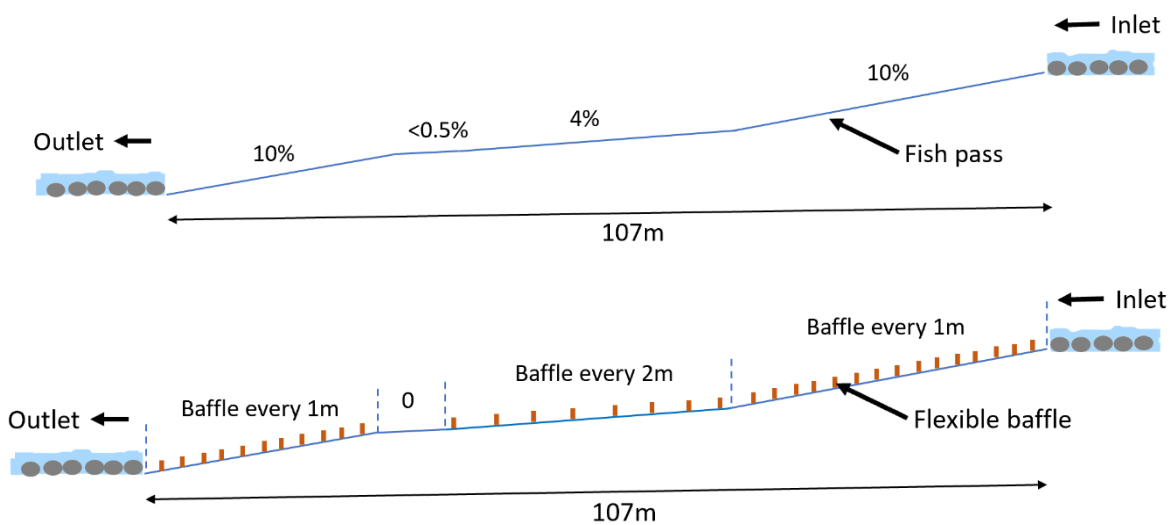
Figure 4. Cross sections of the Saxton Creek fish pass showing the changes in gradient (top) and the spacings between baffles (bottom)
